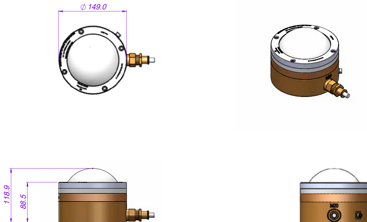
Dimensions (mm)
